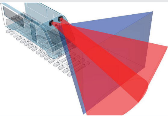
RailScan System
